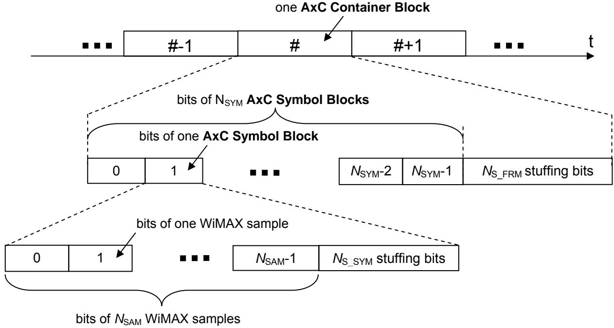
Figure 13C: Symbol based mapping in an AxC Container Block
