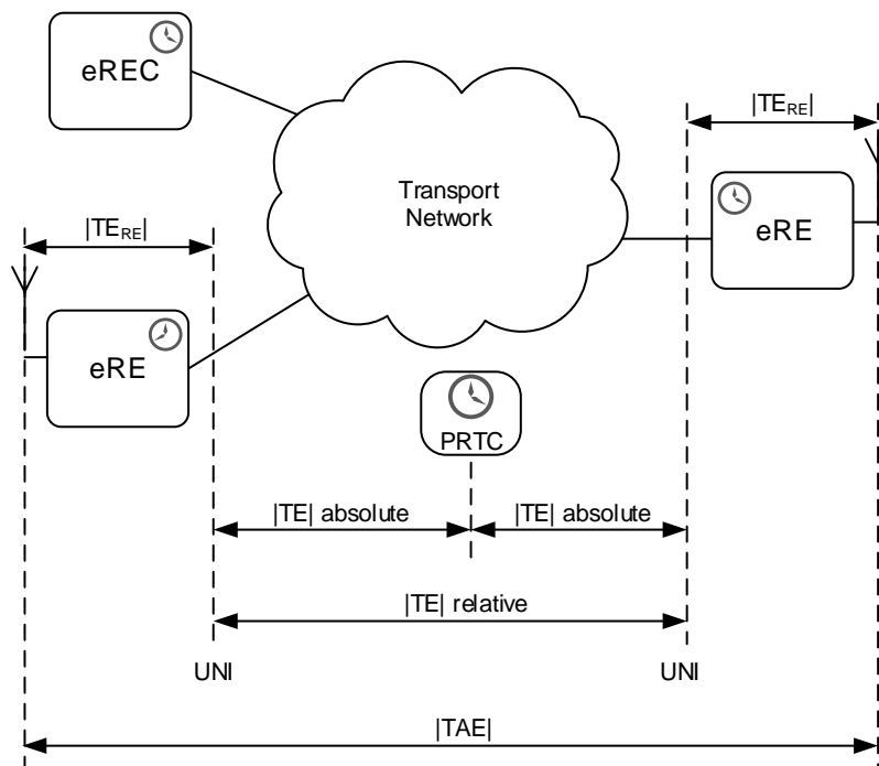
Figure 7 Timing accuracy definitions
